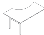
BOY18 1800 / 1200 / 740 43,5 kg
